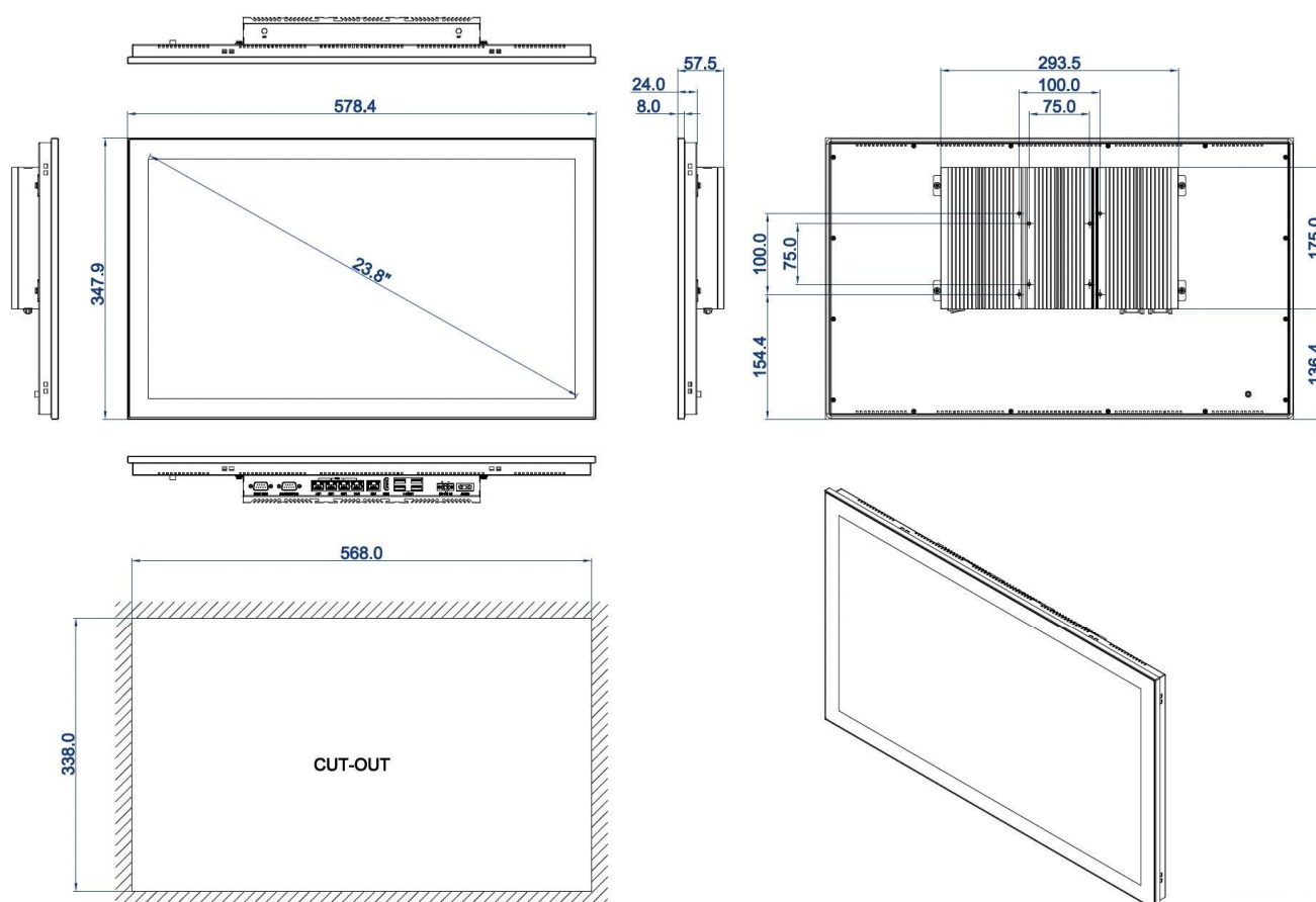
DIMENSIONAL DRAWING:TPC-DCP238T
