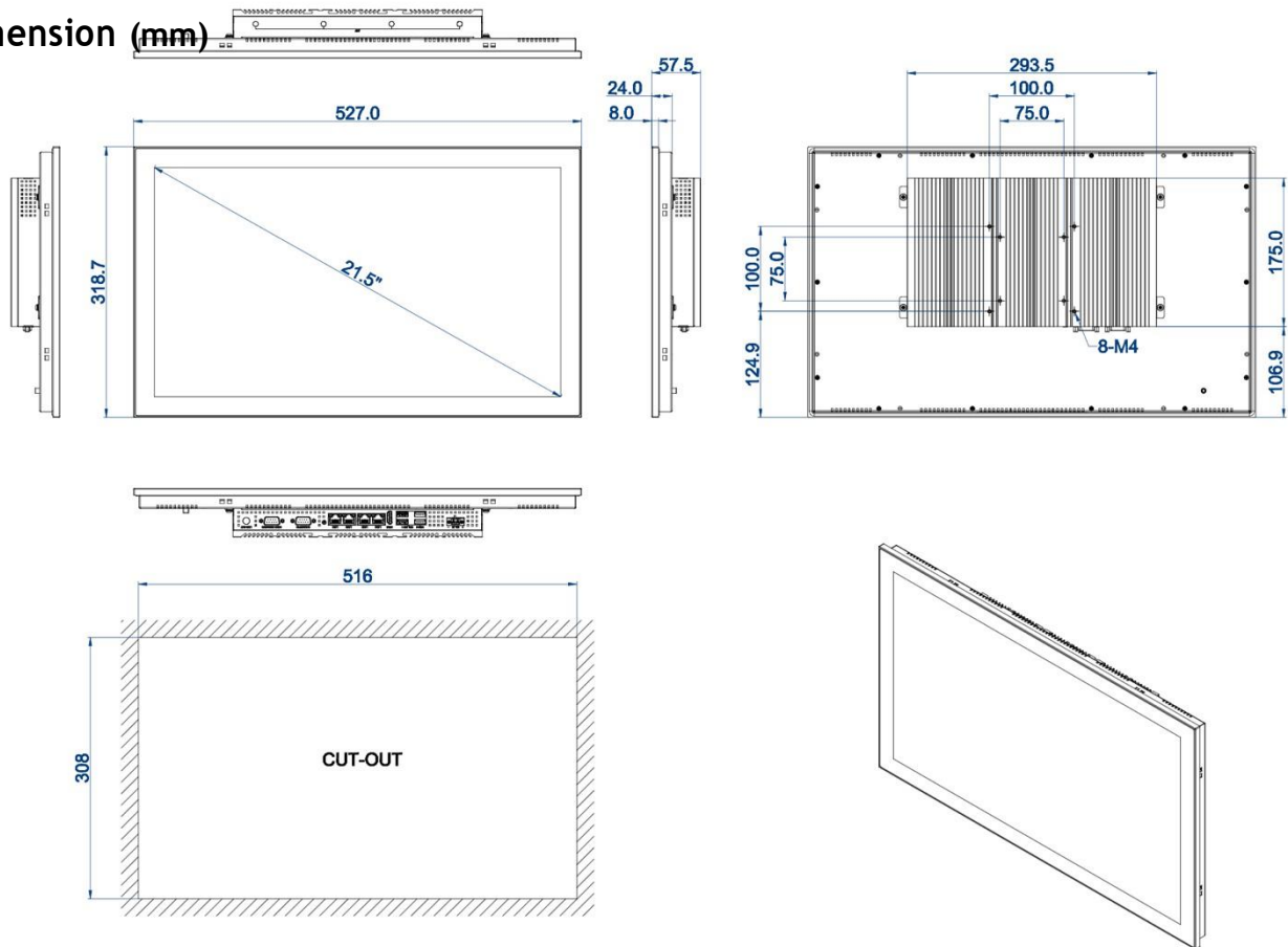
DIMENSIONAL DRAWING:TPC-DCS215E1/N1-4L
